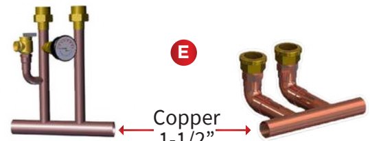
UCS 240 Manifold
